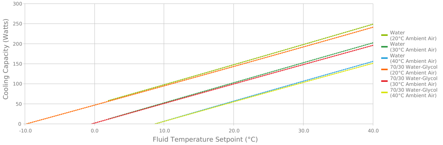
MRC150-DH2-DV \Delta T (Inlet-Outlet) Fluid Temperature
