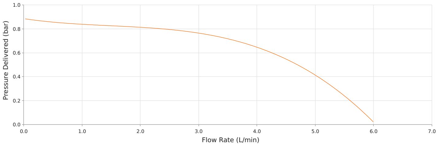
MRC150-DH2-DV - Pump Capacity
