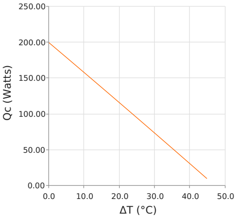
Heat Pumped at Cold Side (Qc) Voperating = 24.01 Volts | Ioperating = 7.96 Amps
