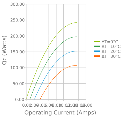
Heat Pumped at Cold Side ( Q_c ) T_{ambient} = 35^{\circ}C | T_{control} = 20^{\circ}C
