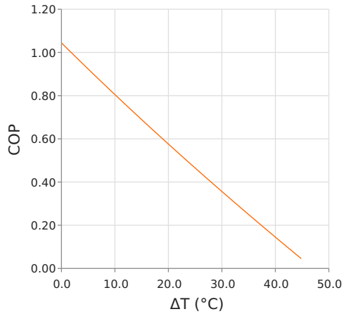
Coefficient of Performance (COP = Qc/Pin) Voperating = 24.01 Volts | Ioperating = 7.96 Amps
