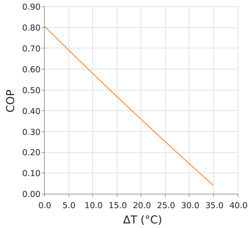
Coefficient of Performance (COP = Qc/Pin) Voperating = 24.02 Volts | Ioperating = 7.59 Amps
