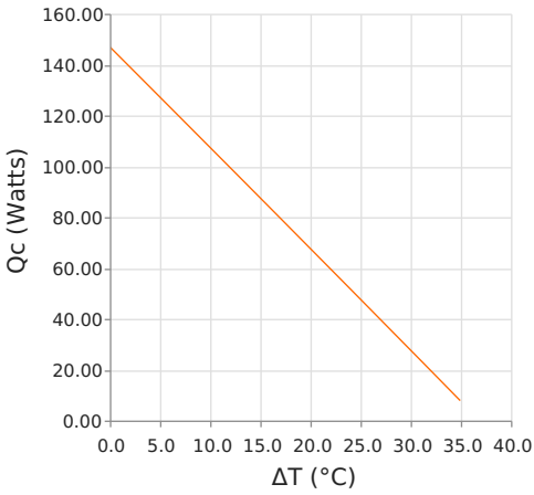
Heat Pumped at Cold Side (Qc) Voperating = 24.02 Volts | Ioperating = 7.59 Amps
