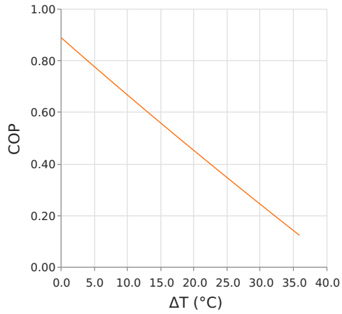
Coefficient of Performance (COP = Qc/Pin) Voperating = 24.06 Volts | Ioperating = 3.73 Amps
