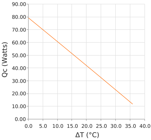
Heat Pumped at Cold Side (Qc) Voperating = 24.06 Volts | Ioperating = 3.73 Amps
