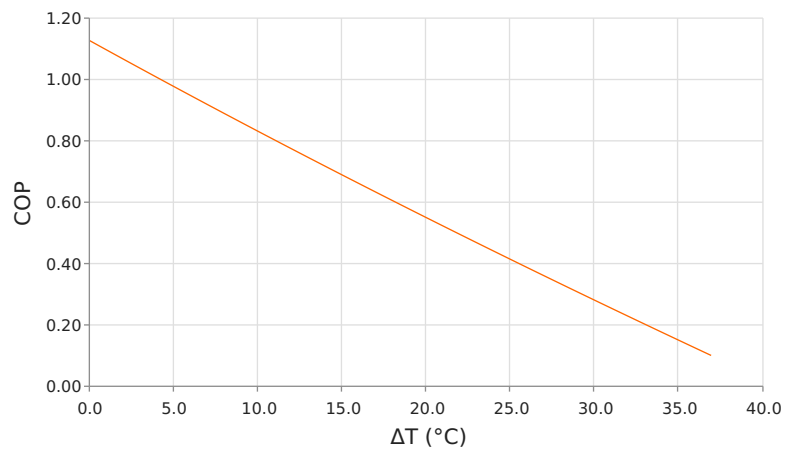
Coefficient of Performance (COP = Q_c/P_{in} ) V_{operating} = 48.15\text{ Volts} | I_{operating} = 8.84\text{ Amps}
