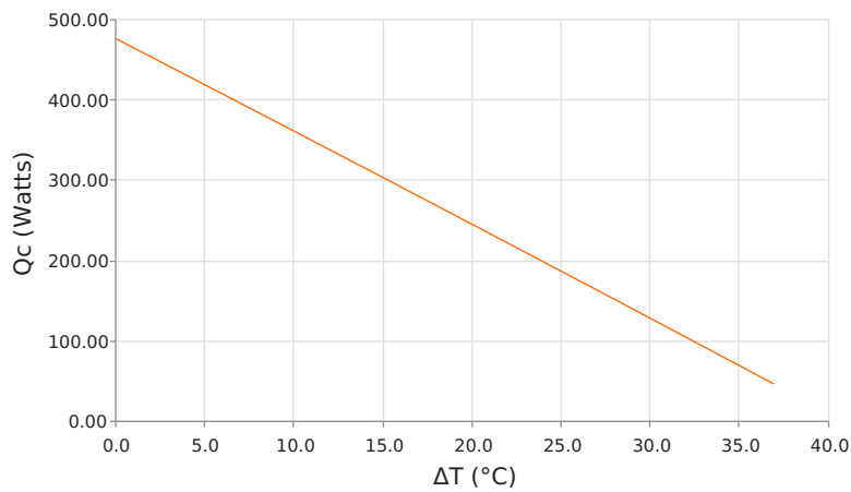
Heat Pumped at Cold Side ( Q_c ) V_{operating} = 48.15\text{ Volts} | I_{operating} = 8.84\text{ Amps}
